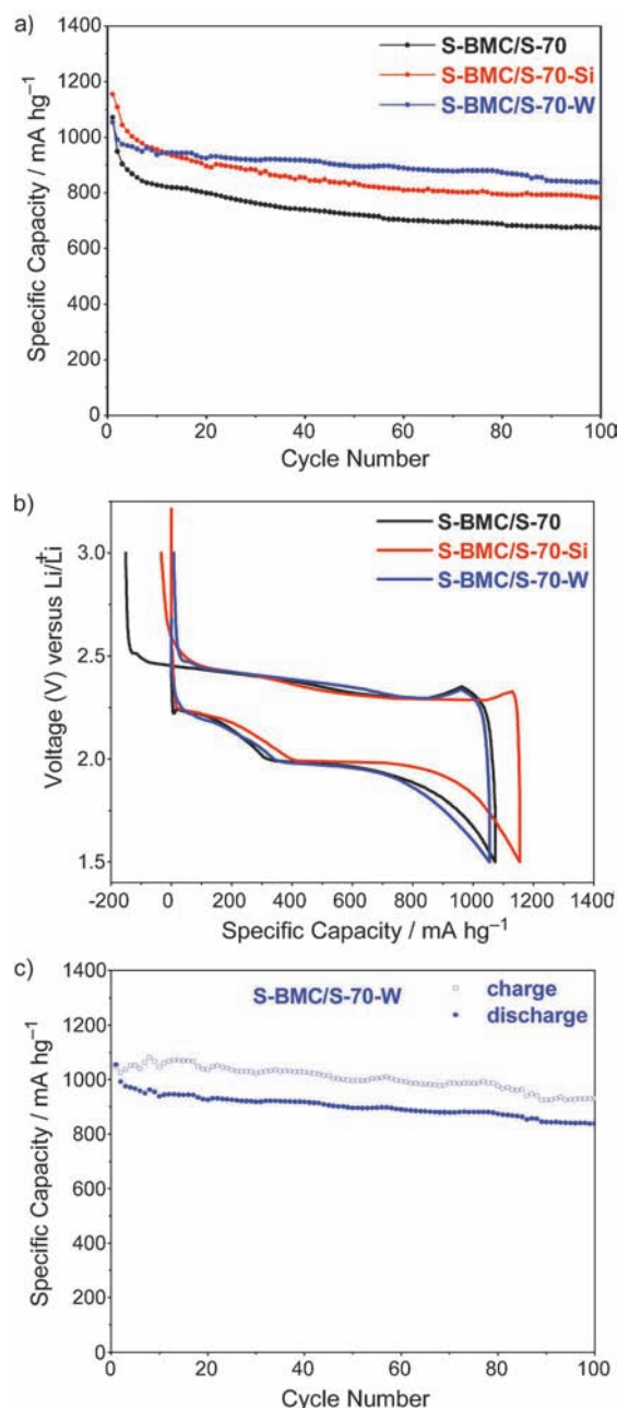
Figure 3. a) Cycling stability of the three 70 wt % C/S electrodes, as prepared (S-BMC/S-70), washed (S-BMC/S-70-W) and SiO x -coated (S-BMC/S-70-Si). b) Comparison of initial charge–discharge profiles of as-prepared S-BMC/S-70 versus post-treated samples by SiO x coating or CS 2 washing. c) Discharge and charge capacity of S-BMC/S-70-W as a function of cycle number. All the cells were operated at a current rate of 1 C (1675 mA g -1 ) at room temperature.
